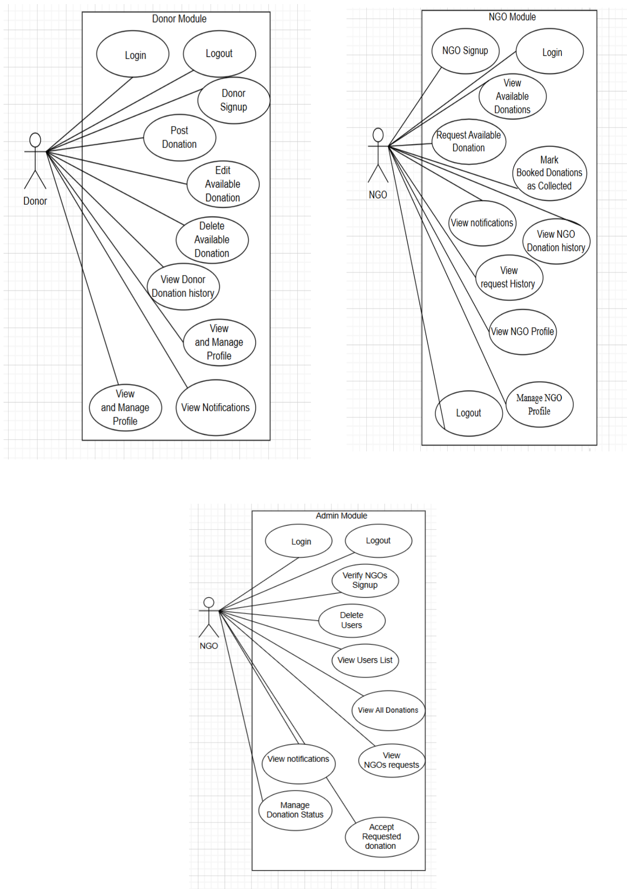
Figure 2.2: Usecase diagram
