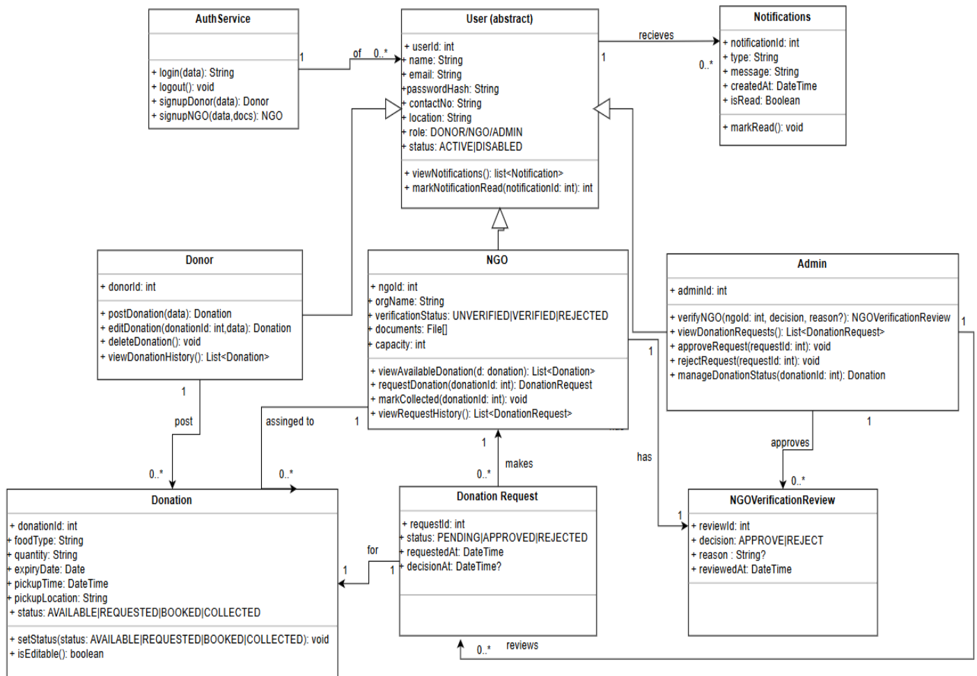
Figure 3.1: Class Diagram
